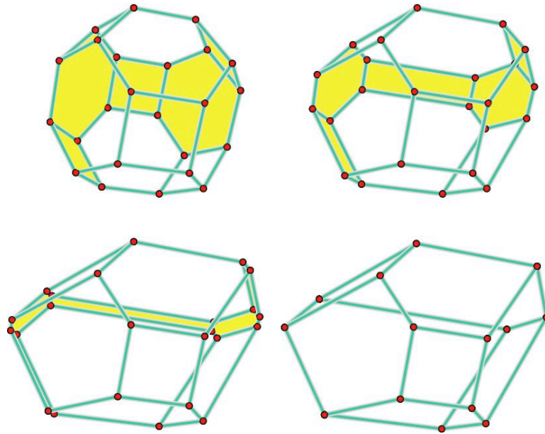
FIGURE 7. The facets that correspond to non-admissible inequalities for the non-symmetric orientation \mathcal{A} of Figure 2 (right associahedron) are colored (the perspective has changed by roughly 90 degrees with respect to the vertical direction for a better visualization). The four pictures show the process of removing these hyperplanes from the A_3 -permutahedron (upper left) to the associahedron (bottom right).
