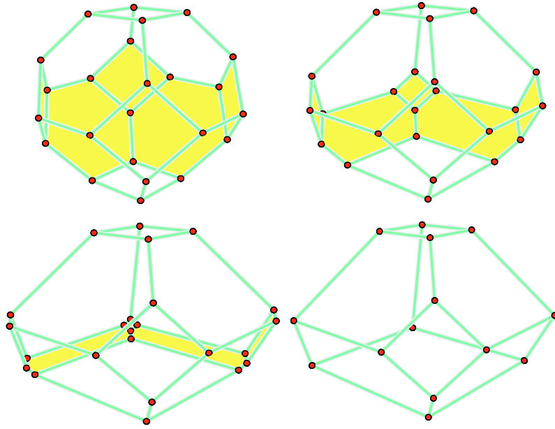
FIGURE 6. The facets that correspond to non-admissible inequalities for the symmetric orientation \mathcal{A} of Figure 2 (left associahedron) are colored. The four pictures show the process of removing these hyperplanes from the A_3 -permutahedron (upper left) to the associahedron (bottom right).
